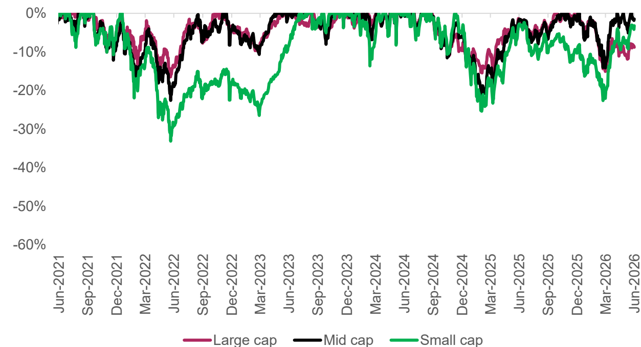
Maximum Drawdown
